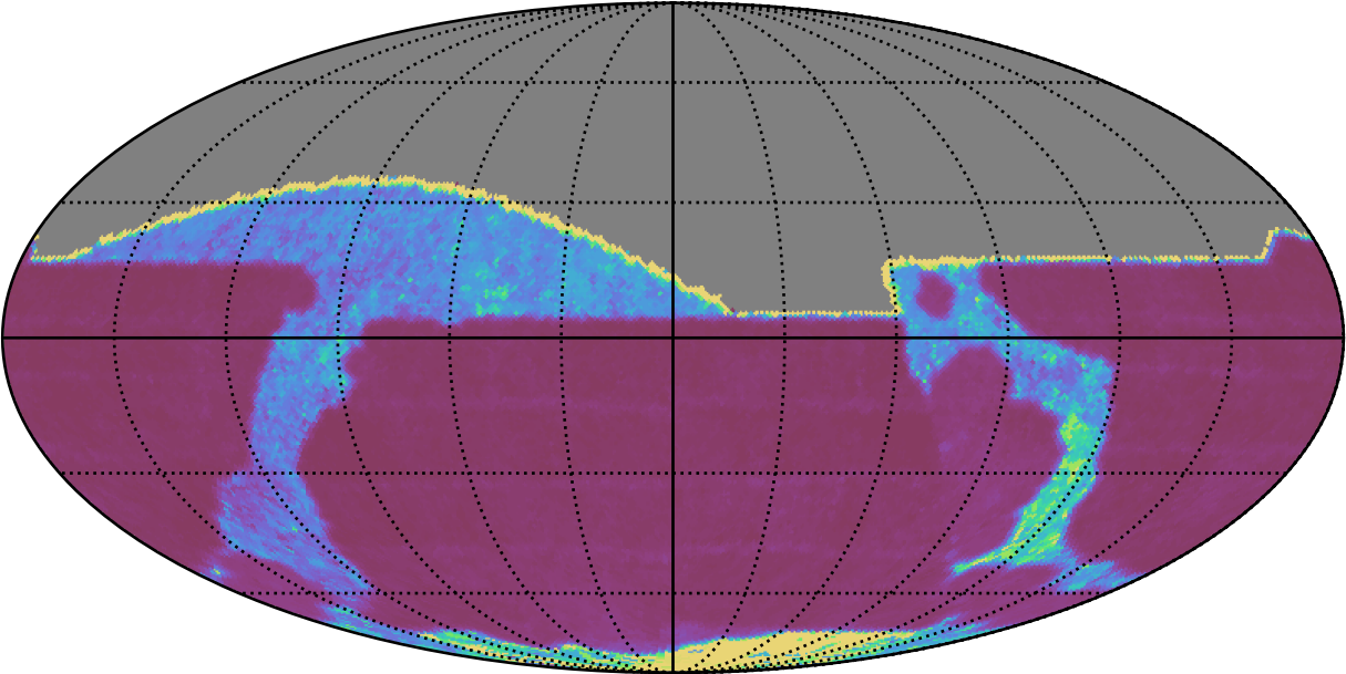
roll_uniform_eh_acc0.5_mjdp0_v3.4_10yrs All sky r band: Median Inter-Night Gap
