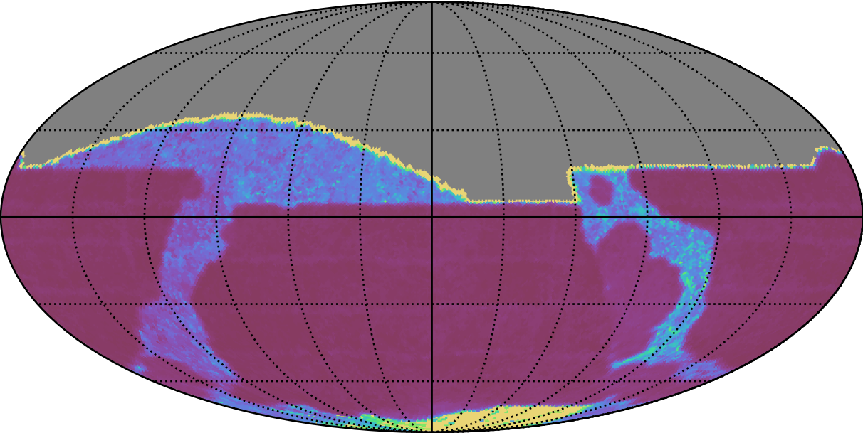
roll_uniform_eh_acc0.5_mjdp0_v3.4_10yrs All sky i band: Median Inter-Night Gap
