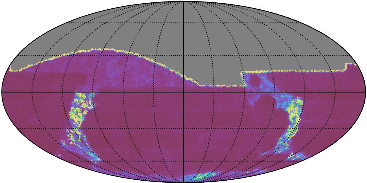
roll_uniform_eh_acc0.5_mjdp0_v3.4_10yrs All sky g band: Median Inter-Night Gap
