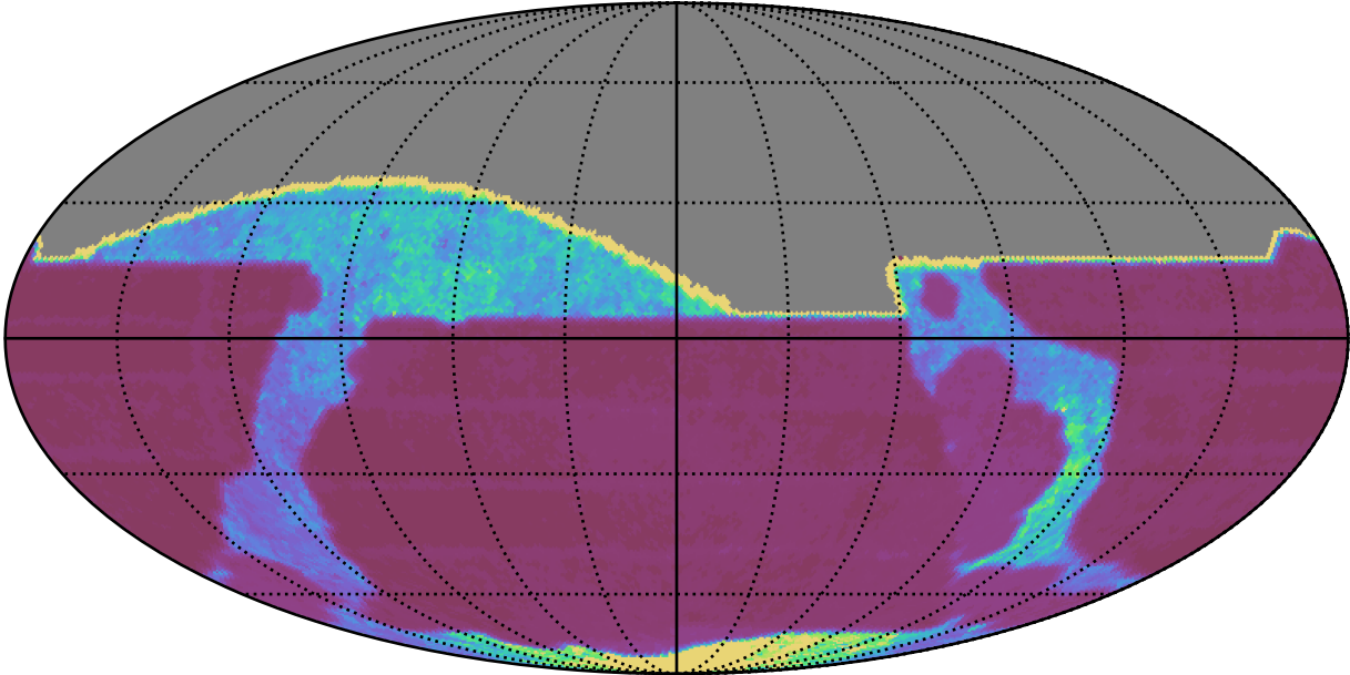
roll_uniform_eh_acc0.5_mjdp0_v3.4_10yrs All sky all bands: Median Inter-Night Gap
