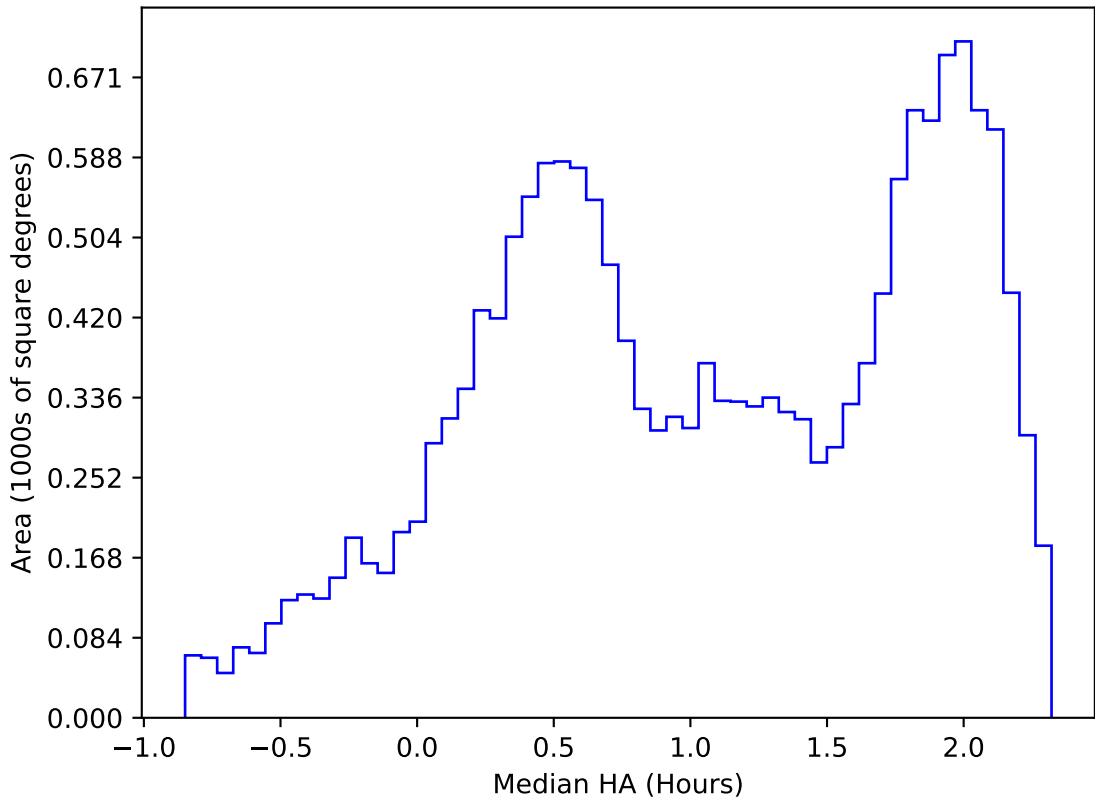
roll_uniform_eh_acc0.5_mjdp0_v3.4_10yrs WFD z band: Median HA
