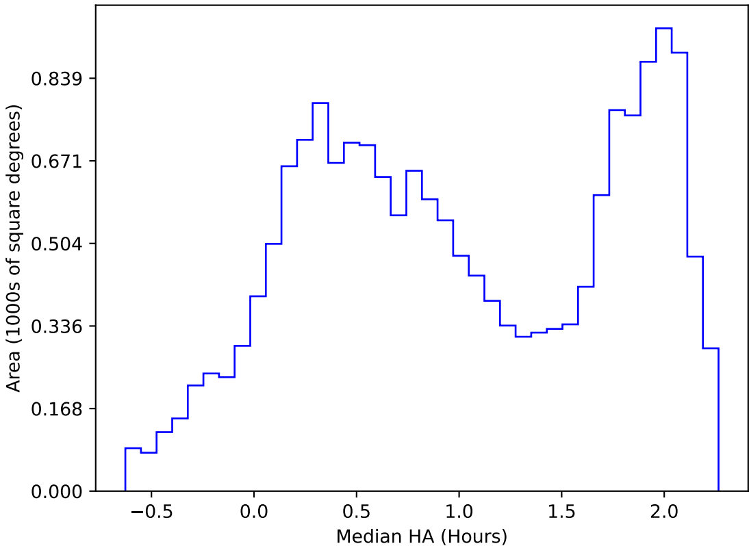
roll_uniform_eh_acc0.5_mjdp0_v3.4_10yrs WFD i band: Median HA
