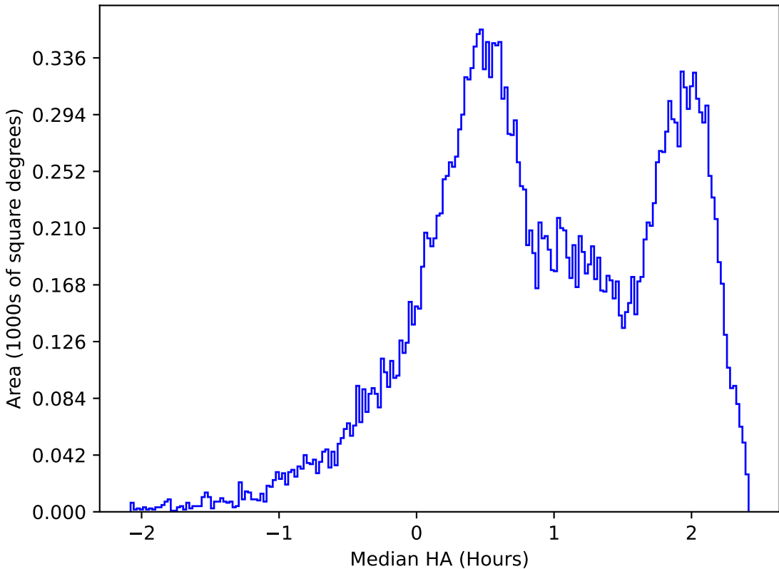
roll_uniform_eh_acc0.5_mjdp0_v3.4_10yrs All sky z band: Median HA
