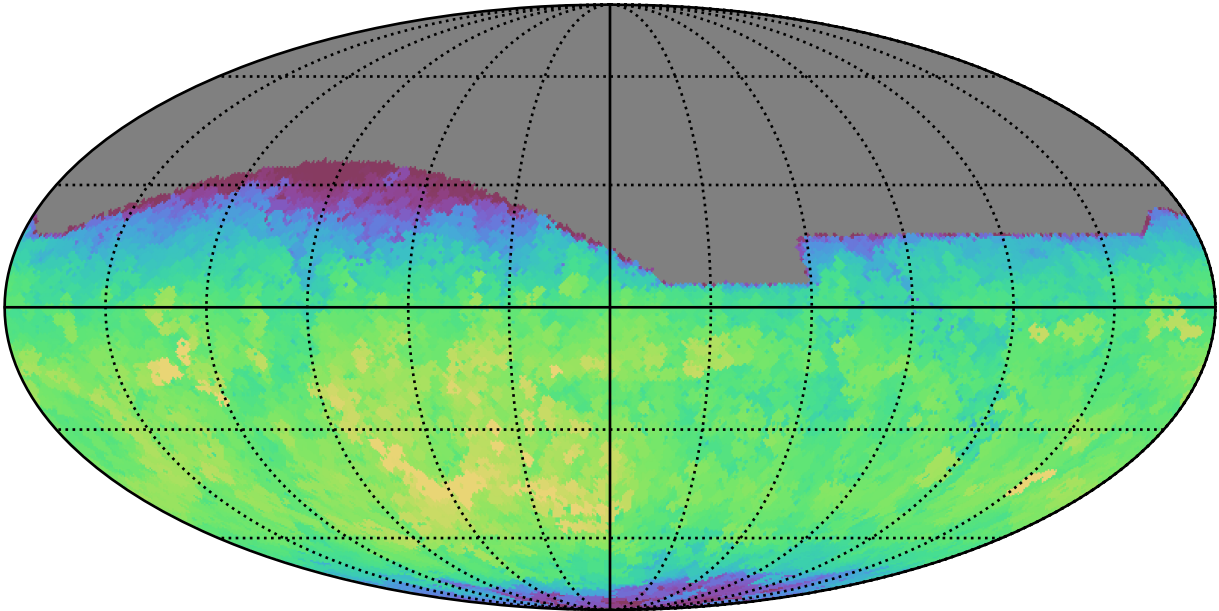
roll_uniform_eh_acc0.5_mjdp0_v3.4_10yrs All sky r band: Max fiveSigmaDepth
