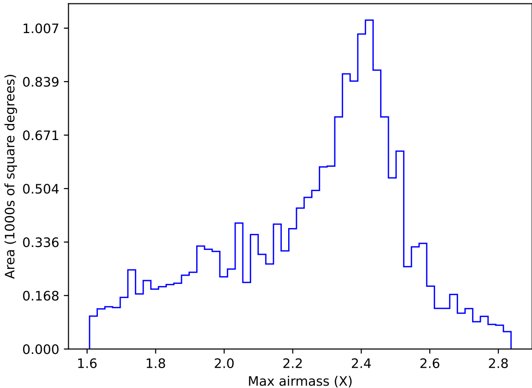
roll_uniform_eh_acc0.5_mjdp0_v3.4_10yrs WFD r band: Max airmass
