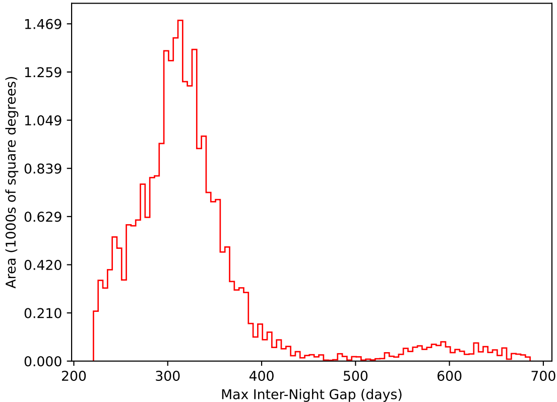
roll_uniform_eh_acc0.5_mjdp0_v3.4_10yrs All sky i band: Max Inter-Night Gap
