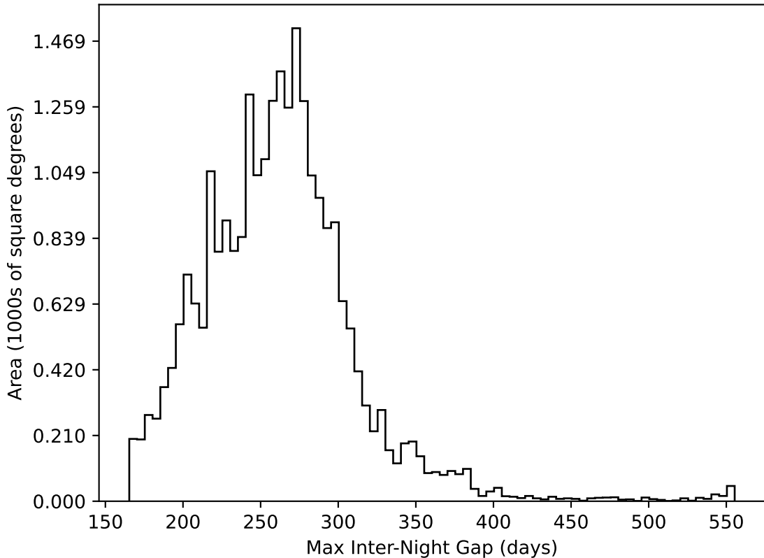
roll_uniform_eh_acc0.5_mjdp0_v3.4_10yrs All sky all bands: Max Inter-Night Gap
