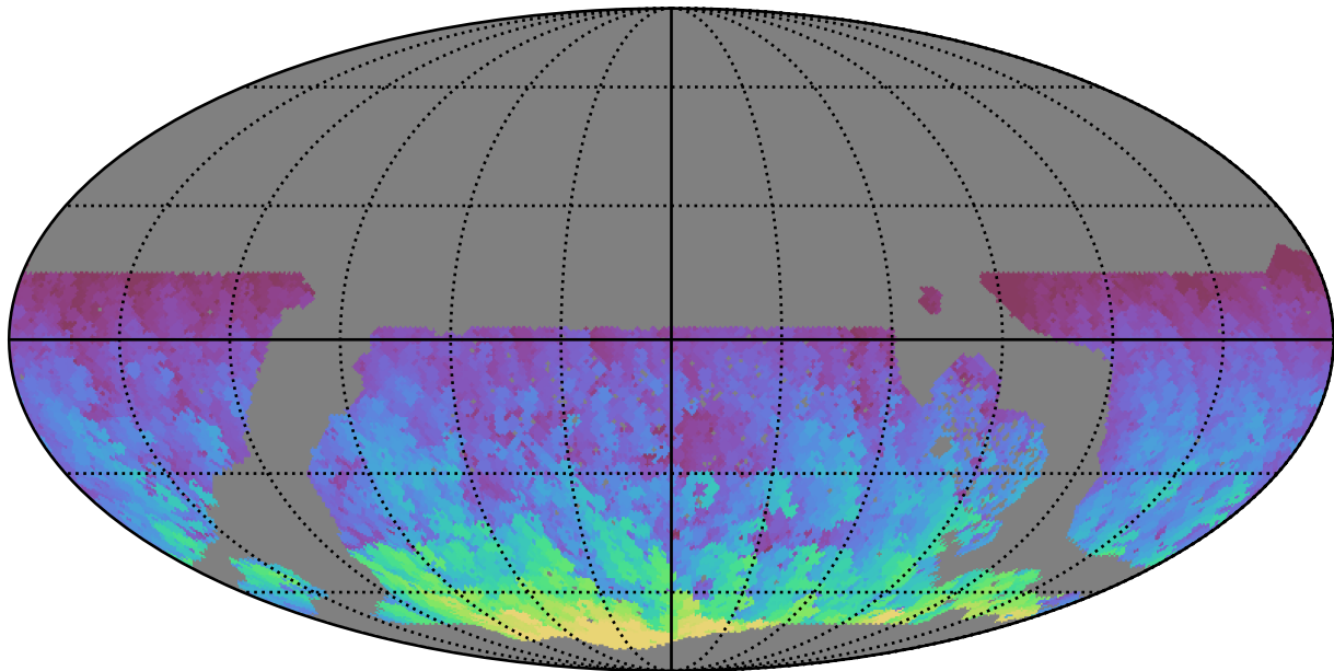
roll_uniform_eh_acc0.5_mjdp0_v3.4_10yrs WFD y band: Max HA
