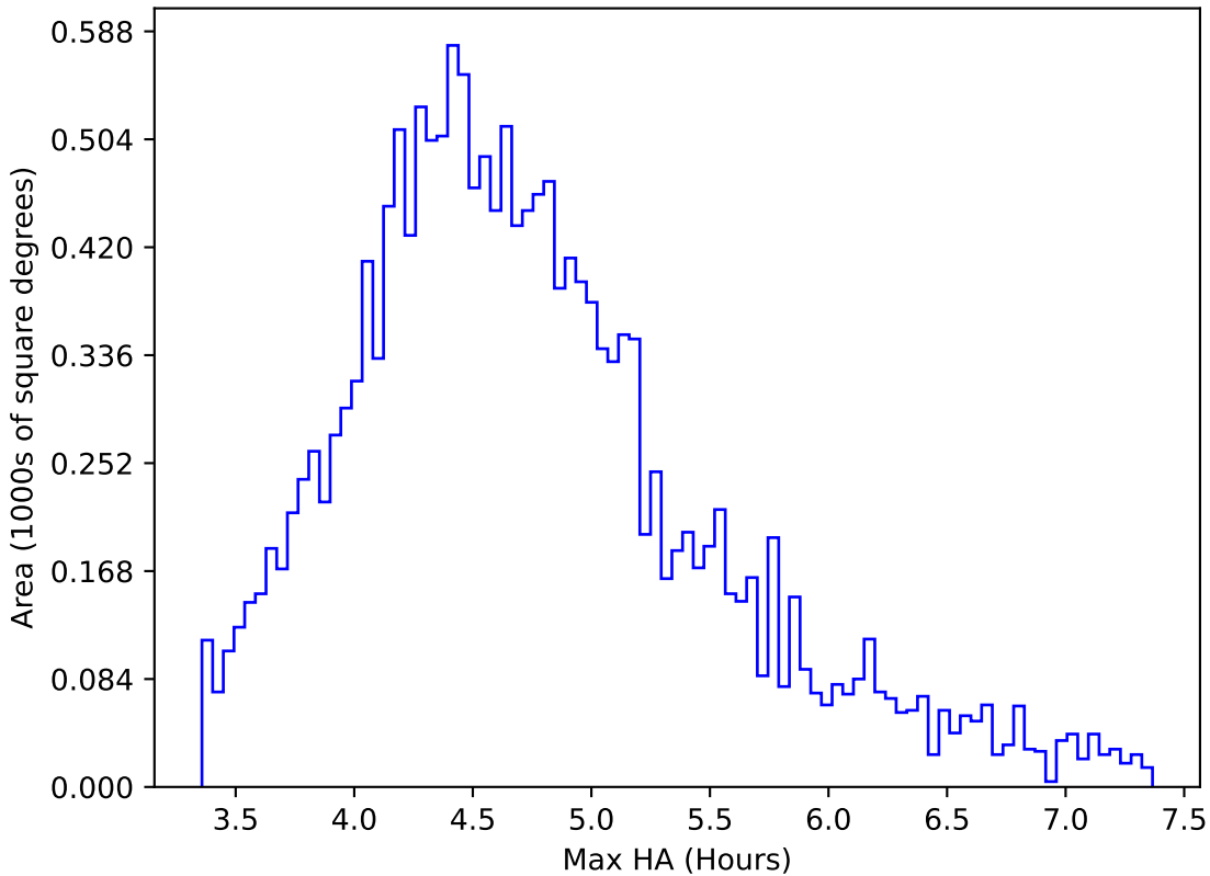
roll_uniform_eh_acc0.5_mjdp0_v3.4_10yrs WFD y band: Max HA
