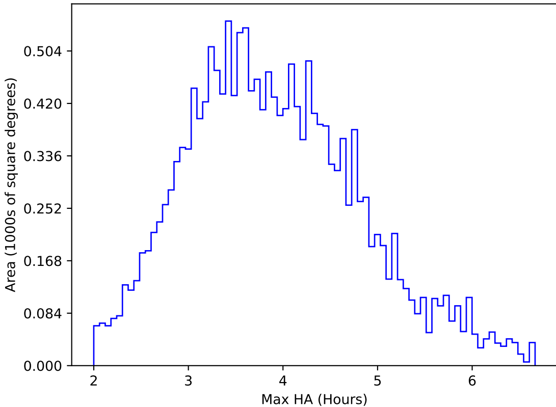
roll_uniform_eh_acc0.5_mjdp0_v3.4_10yrs WFD u band: Max HA
