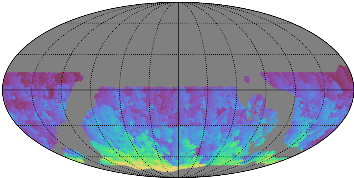
roll_uniform_eh_acc0.5_mjdp0_v3.4_10yrs WFD r band: Max HA
