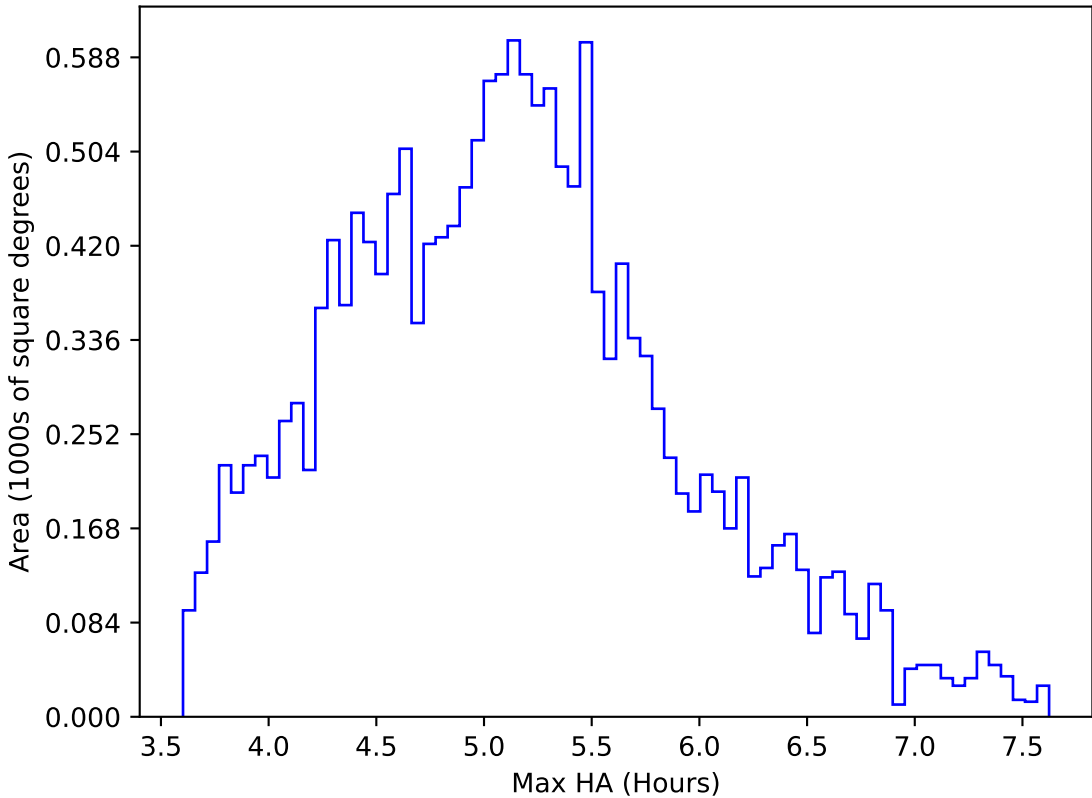
roll_uniform_eh_acc0.5_mjdp0_v3.4_10yrs WFD all bands: Max HA
