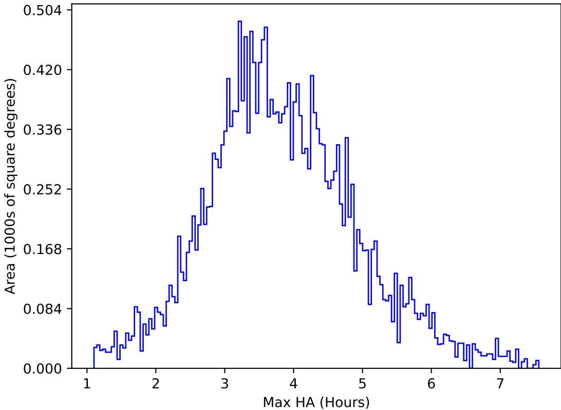
roll_uniform_eh_acc0.5_mjdp0_v3.4_10yrs All sky u band: Max HA
