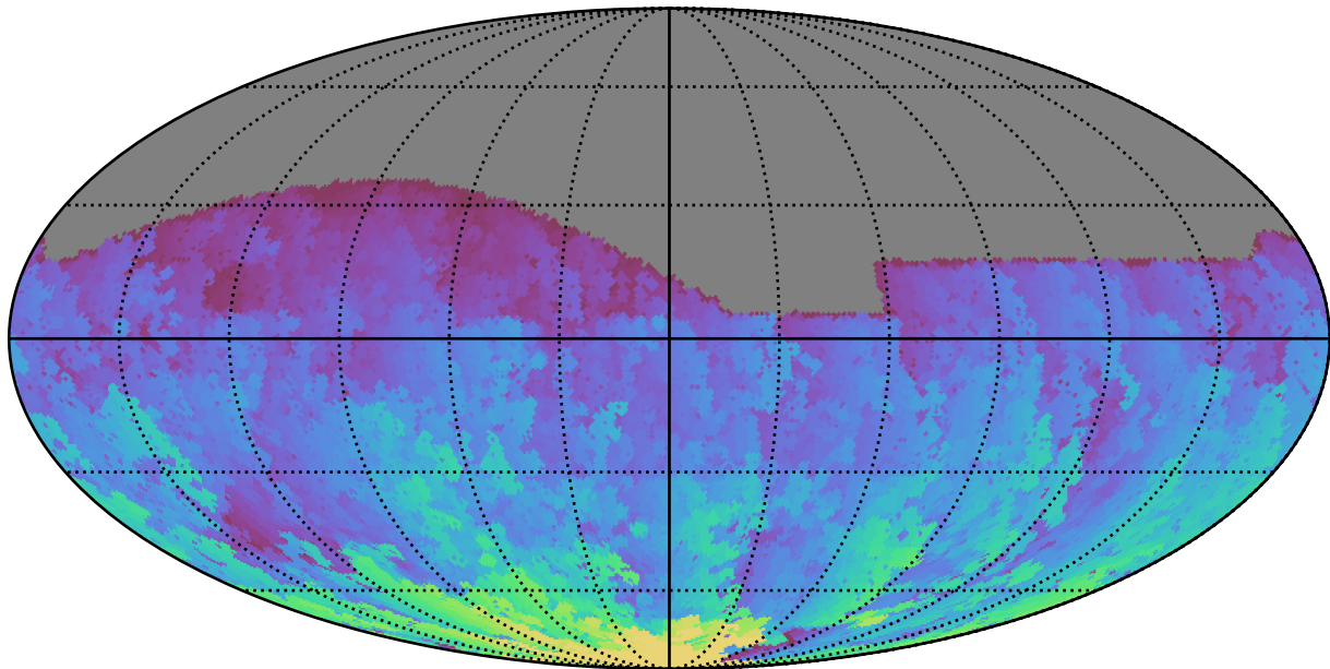
roll_uniform_eh_acc0.5_mjdp0_v3.4_10yrs All sky g band: Max HA
