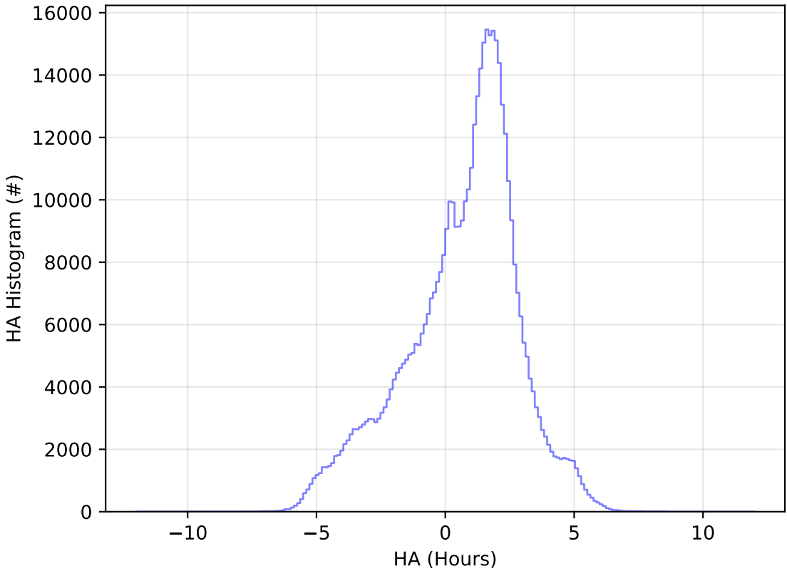
roll_uniform_eh_acc0.5_mjdp0_v3.4_10yrs WFD i band: HA Histogram
