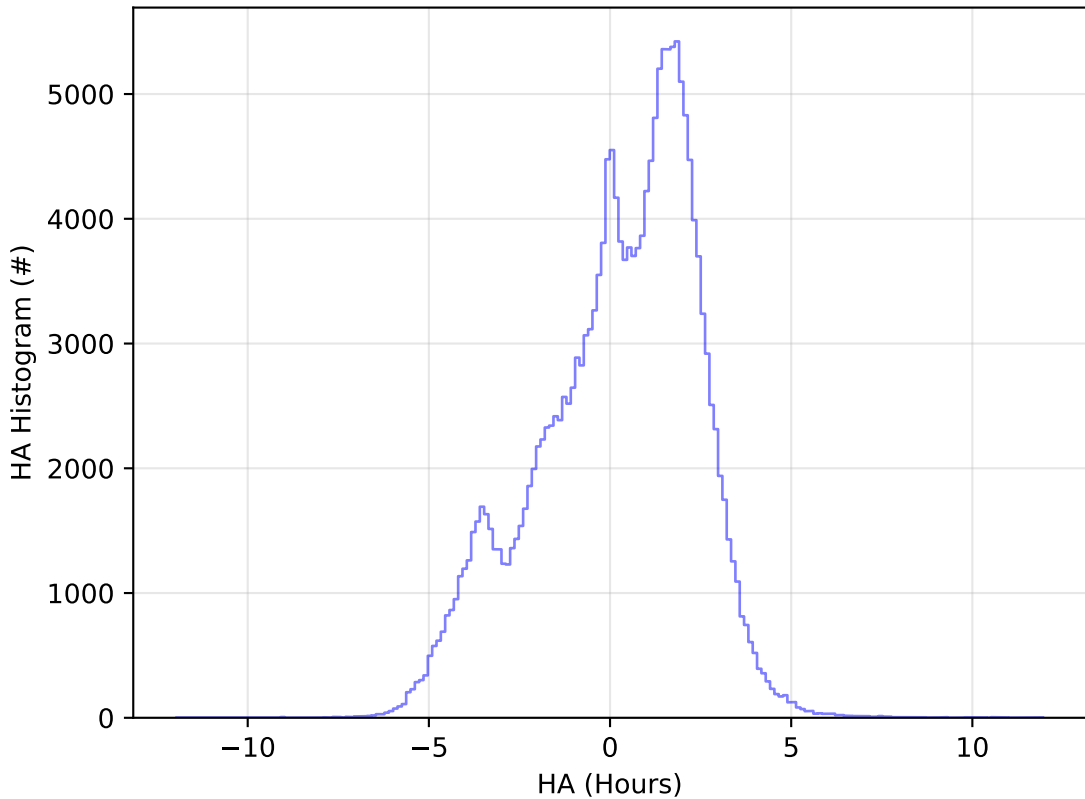
roll_uniform_eh_acc0.5_mjdp0_v3.4_10yrs WFD g band: HA Histogram
