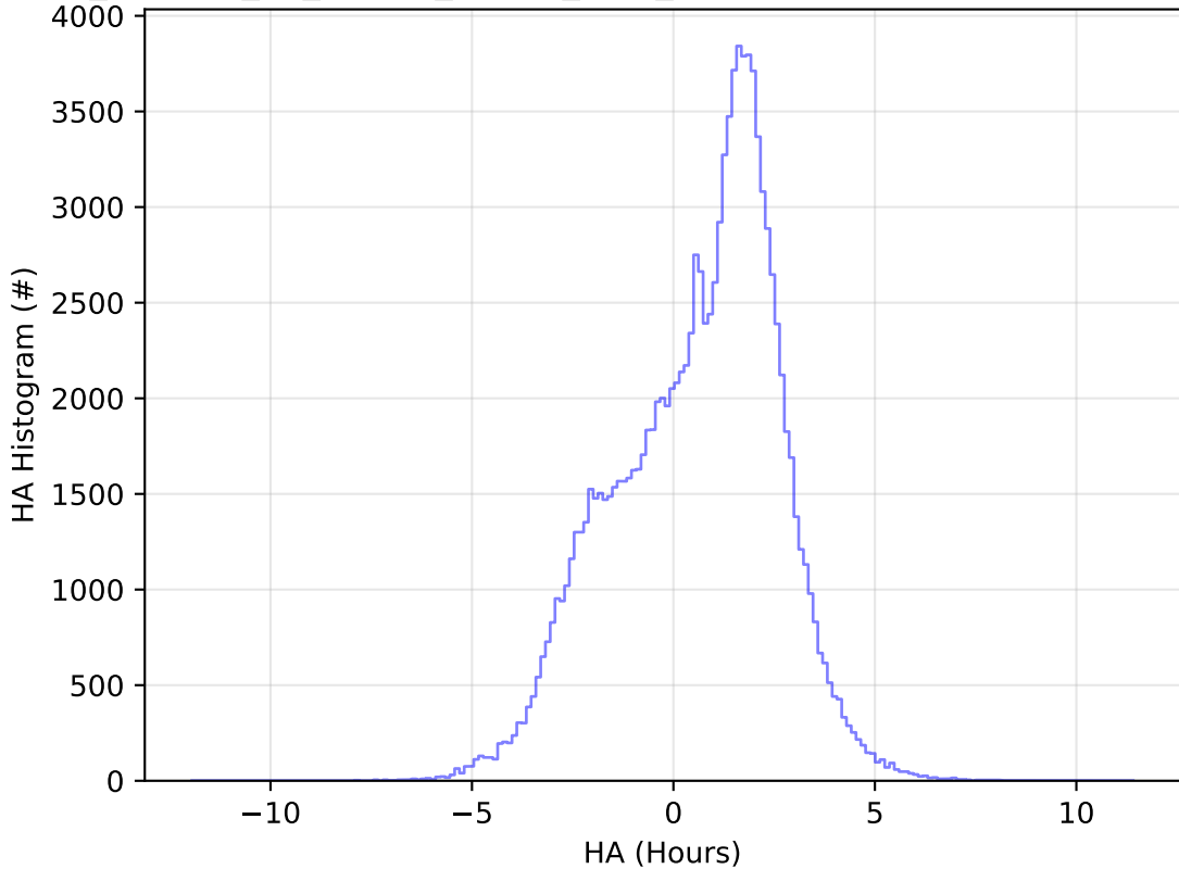
roll_uniform_eh_acc0.5_mjdp0_v3.4_10yrs All sky u band: HA Histogram
