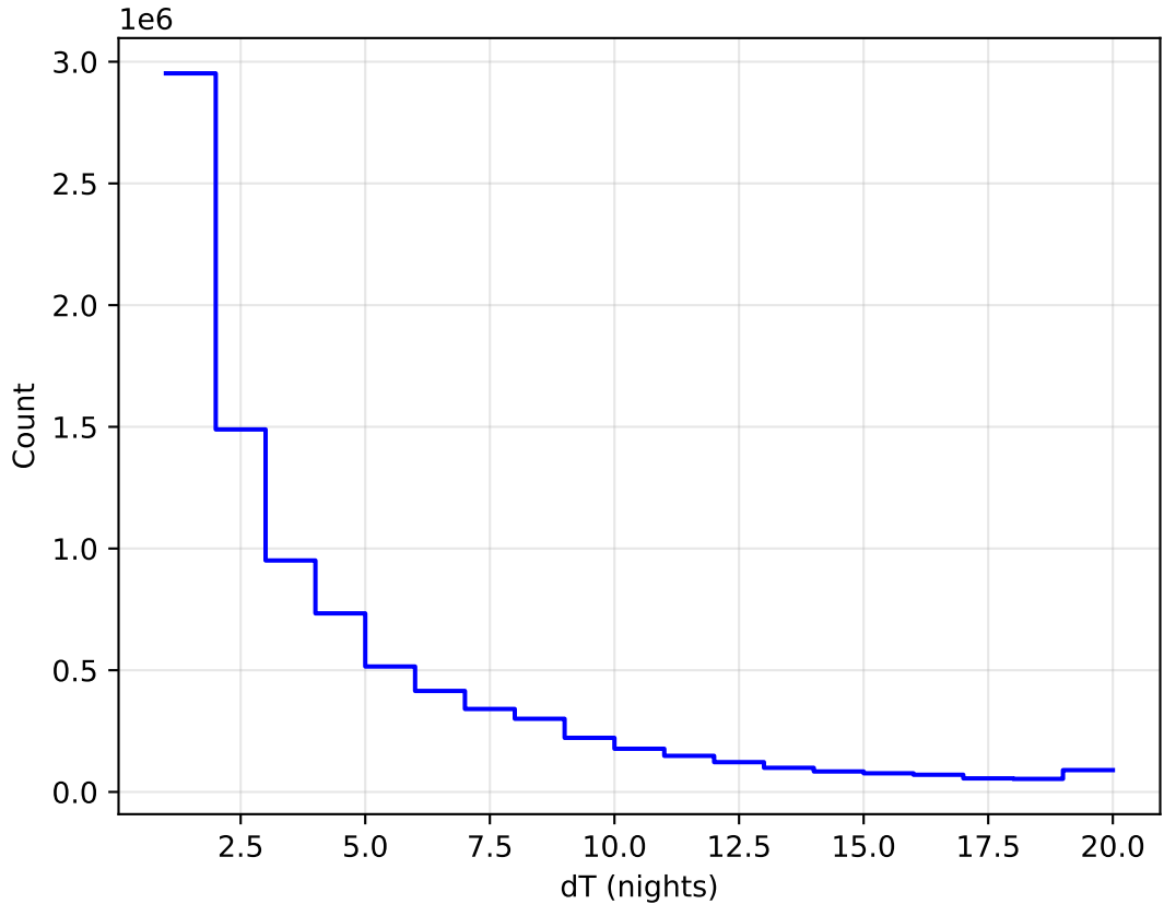
roll_uniform_eh_acc0.5_mjdp0_v3.4_10yrs All sky all bands: DeltaNight Histogram
