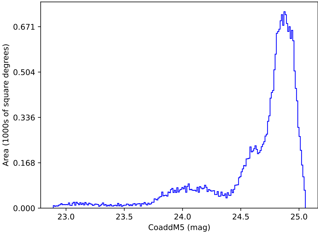
roll_uniform_eh_acc0.5_mjdp0_v3.4_10yrs All sky y band: CoaddM5
