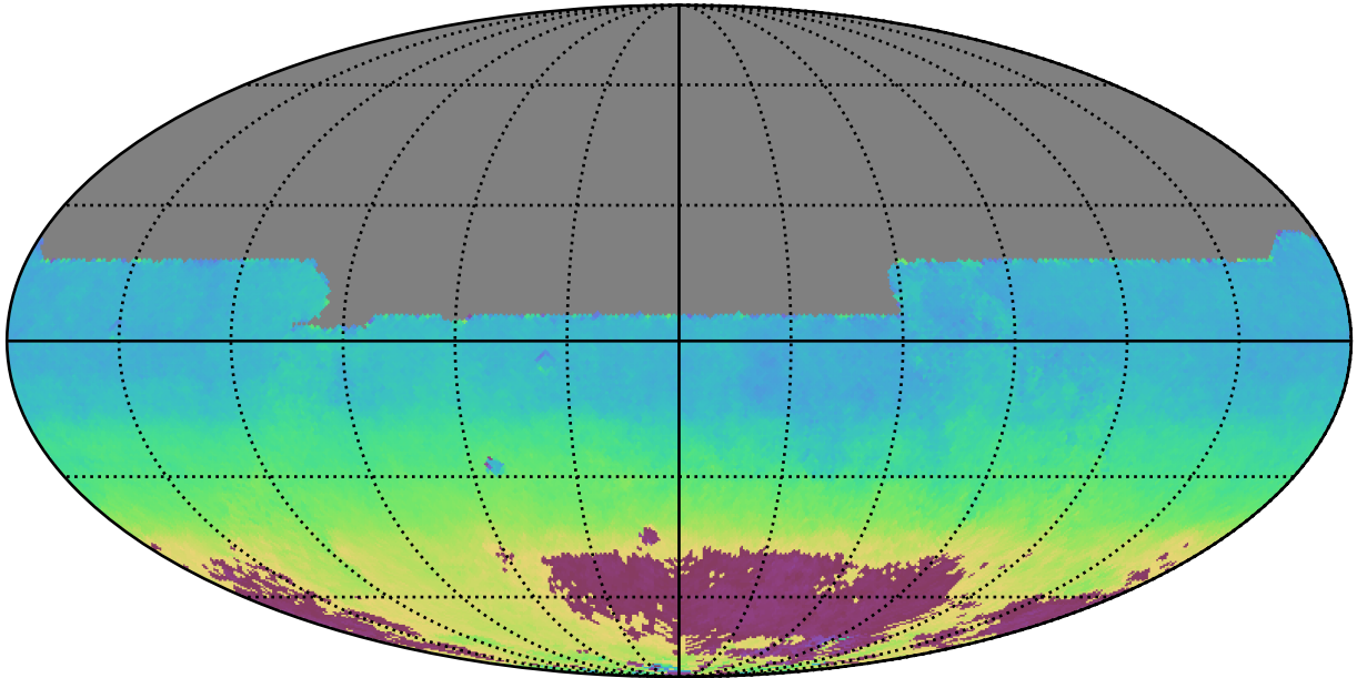
roll_uniform_eh_acc0.5_mjdp0_v3.4_10yrs All sky y band: AngleMean rotSkyPos
