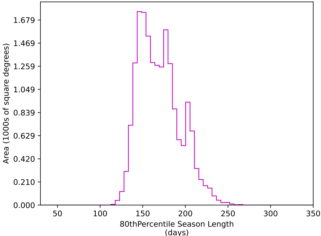
roll_uniform_eh_acc0.5_mjdp0_v3.4_10yrs WFD z band: 80thPercentile Season Length
