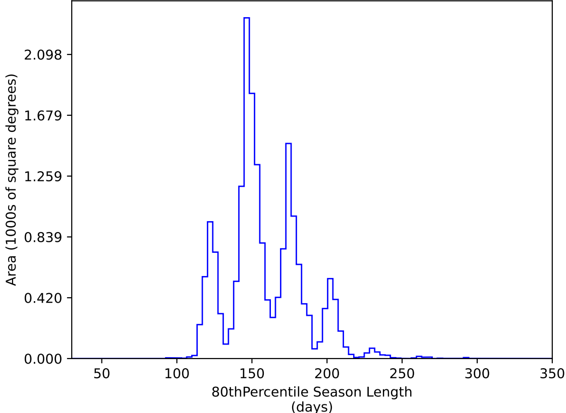
roll_uniform_eh_acc0.5_mjdp0_v3.4_10yrs WFD y band: 80thPercentile Season Length
