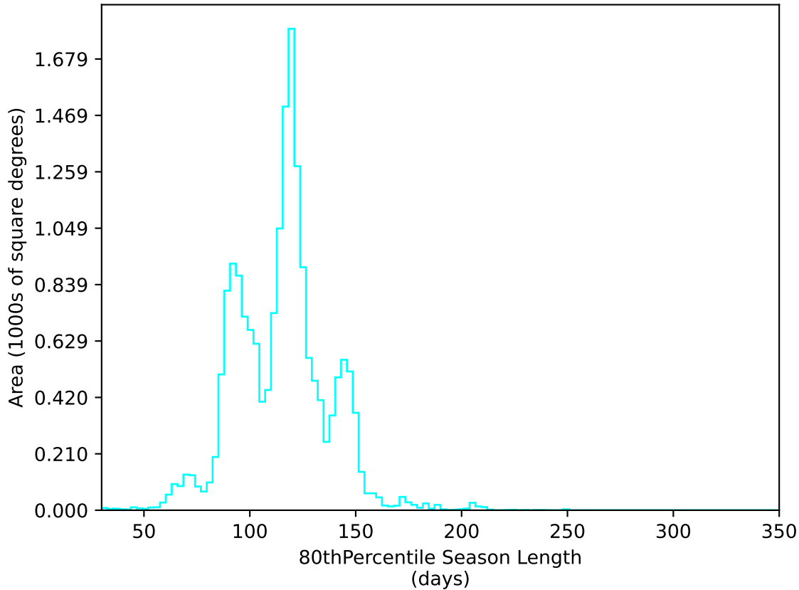
roll_uniform_eh_acc0.5_mjdp0_v3.4_10yrs WFD u band: 80thPercentile Season Length
