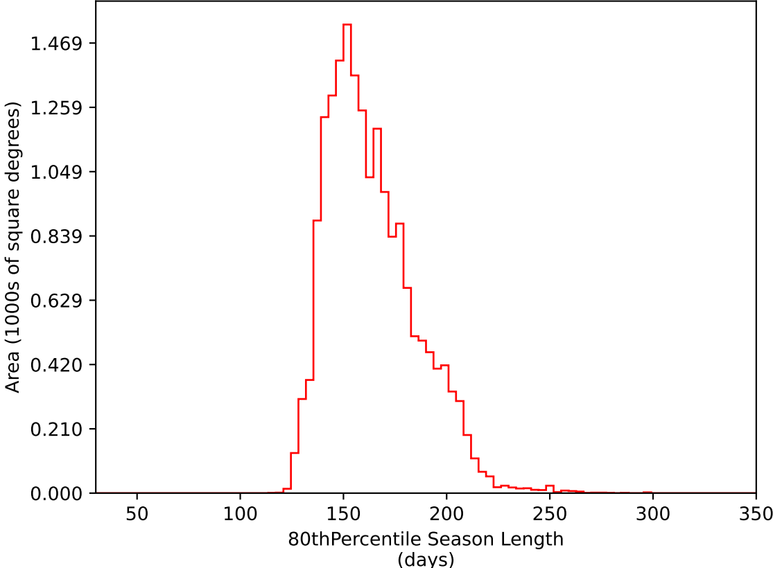
roll_uniform_eh_acc0.5_mjdp0_v3.4_10yrs WFD i band: 80thPercentile Season Length
