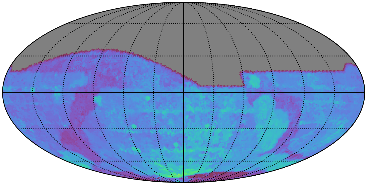
roll_uniform_eh_acc0.5_mjdp0_v3.4_10yrs All sky r band: 80thPercentile Season Length
