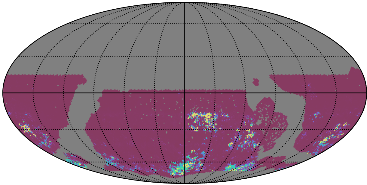
roll_uniform_eh_acc0.5_mjdp0_v3.4_10yrs WFD ri bands: 75th Percentile Intranight Timespan
