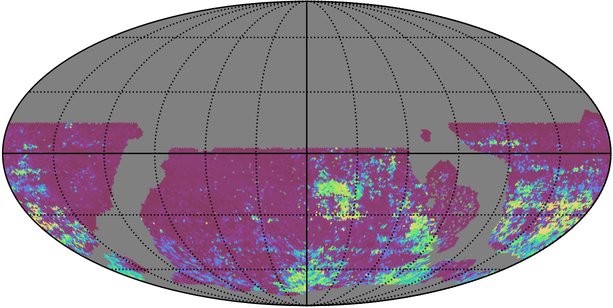
roll_uniform_eh_acc0.5_mjdp0_v3.4_10yrs WFD i band: 75th Percentile Intranight Timespan
