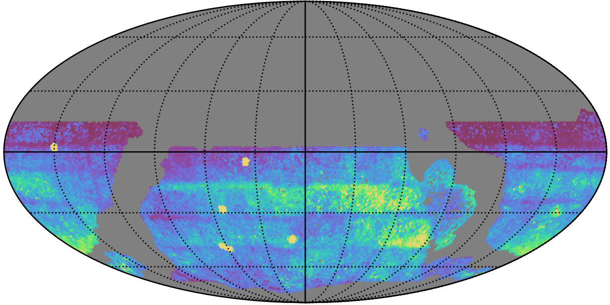
roll_uniform_eh_acc0.5_mjdp0_v3.4_10yrs WFD all bands: 75th Percentile Intranight Timespan
