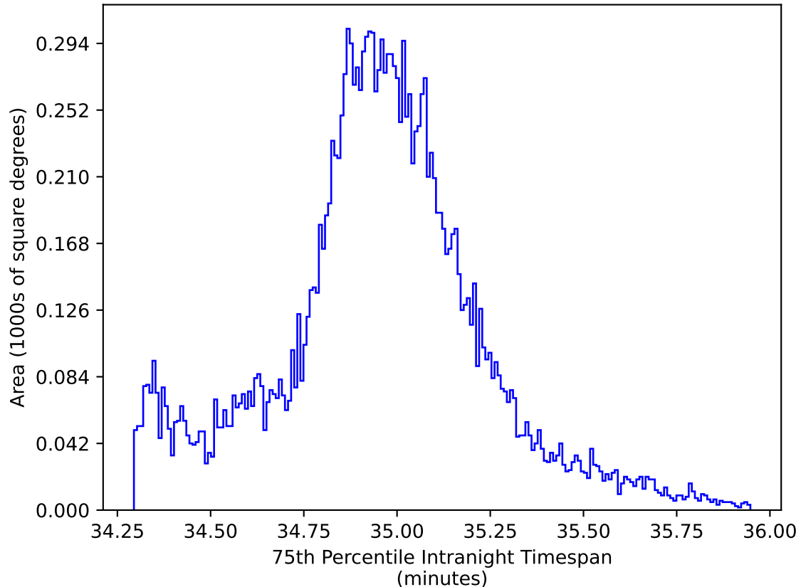
roll_uniform_eh_acc0.5_mjdp0_v3.4_10yrs WFD all bands: 75th Percentile Intranight Timespan
