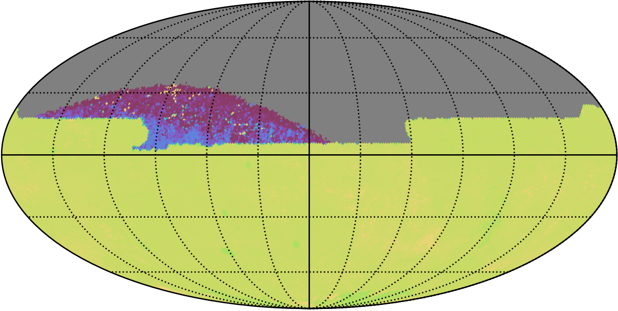
roll_uniform_eh_acc0.5_mjdp0_v3.4_10yrs All sky zy bands: 75th Percentile Intranight Timespan
