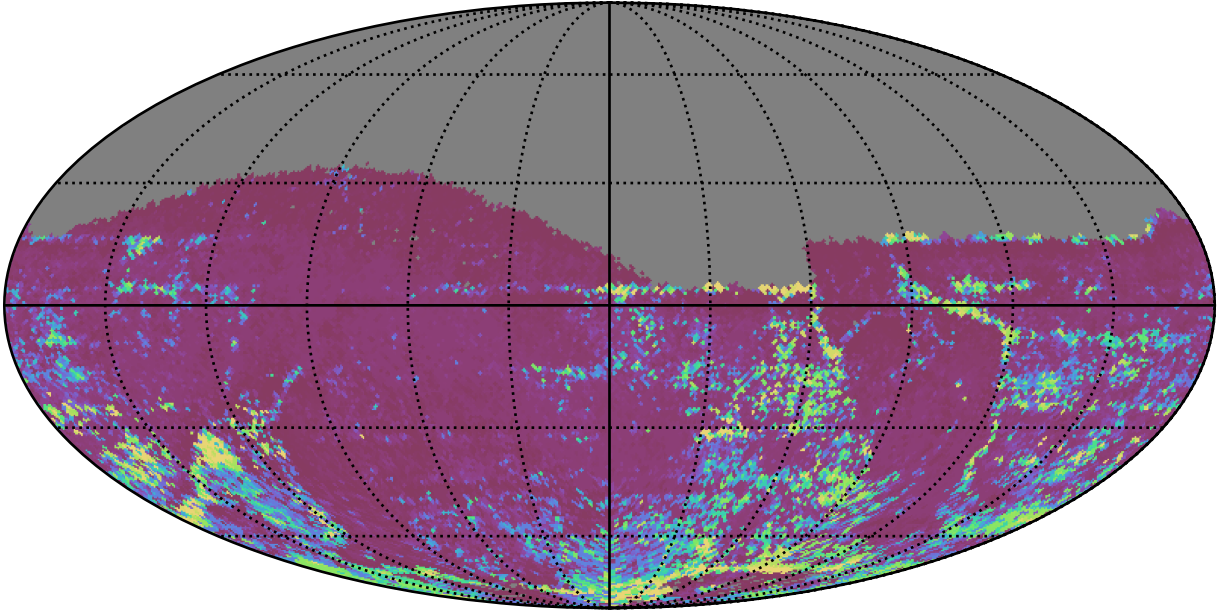
roll_uniform_eh_acc0.5_mjdp0_v3.4_10yrs All sky z band: 75th Percentile Intranight Timespan
