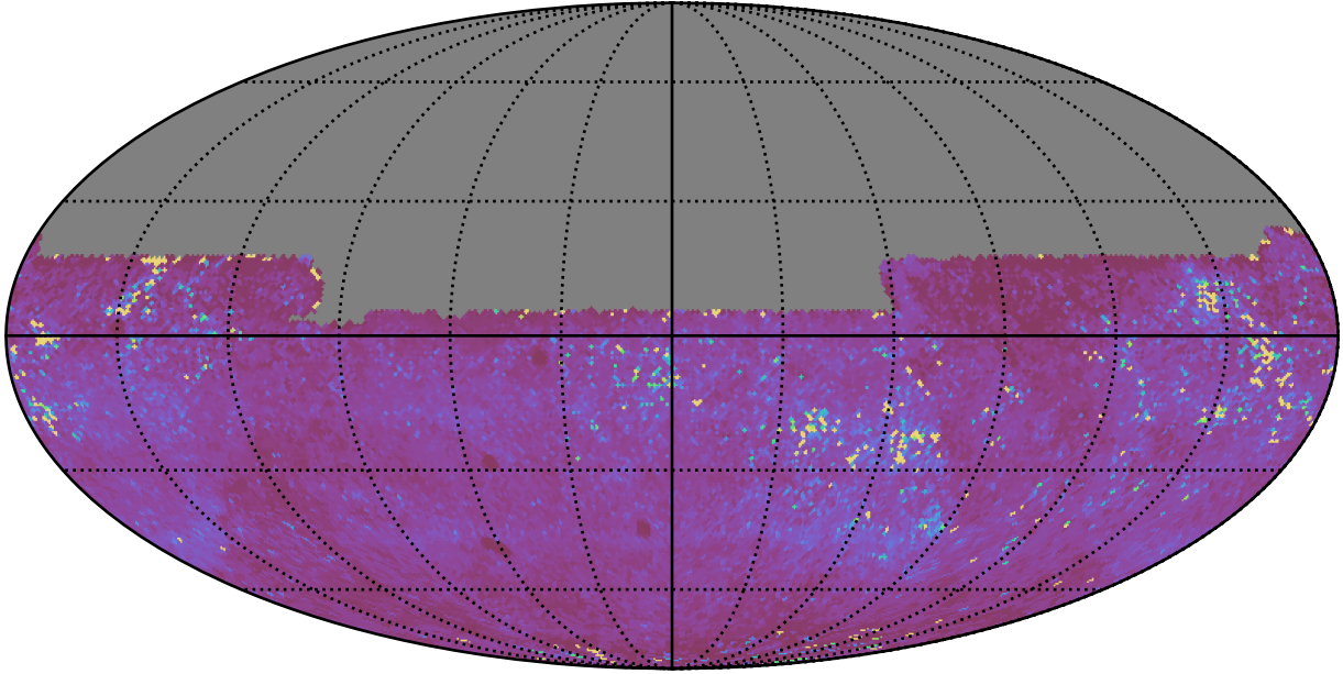
roll_uniform_eh_acc0.5_mjdp0_v3.4_10yrs All sky y band: 75th Percentile Intranight Timespan
