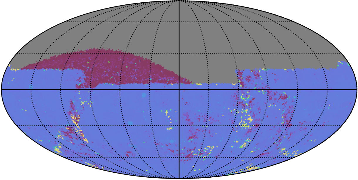
roll_uniform_eh_acc0.5_mjdp0_v3.4_10yrs All sky ug bands: 75th Percentile Intranight Timespan
