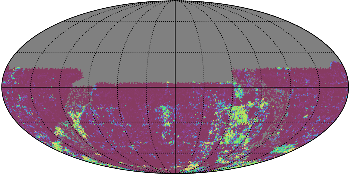
roll_uniform_eh_acc0.5_mjdp0_v3.4_10yrs All sky u band: 75th Percentile Intranight Timespan
