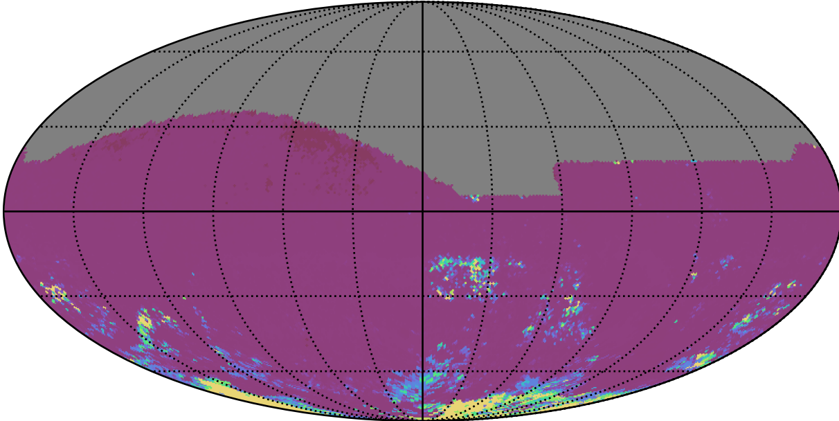
roll_uniform_eh_acc0.5_mjdp0_v3.4_10yrs All sky ri bands: 75th Percentile Intranight Timespan
