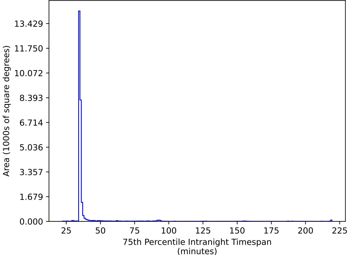
roll_uniform_eh_acc0.5_mjdp0_v3.4_10yrs All sky ri bands: 75th Percentile Intranight Timespan
