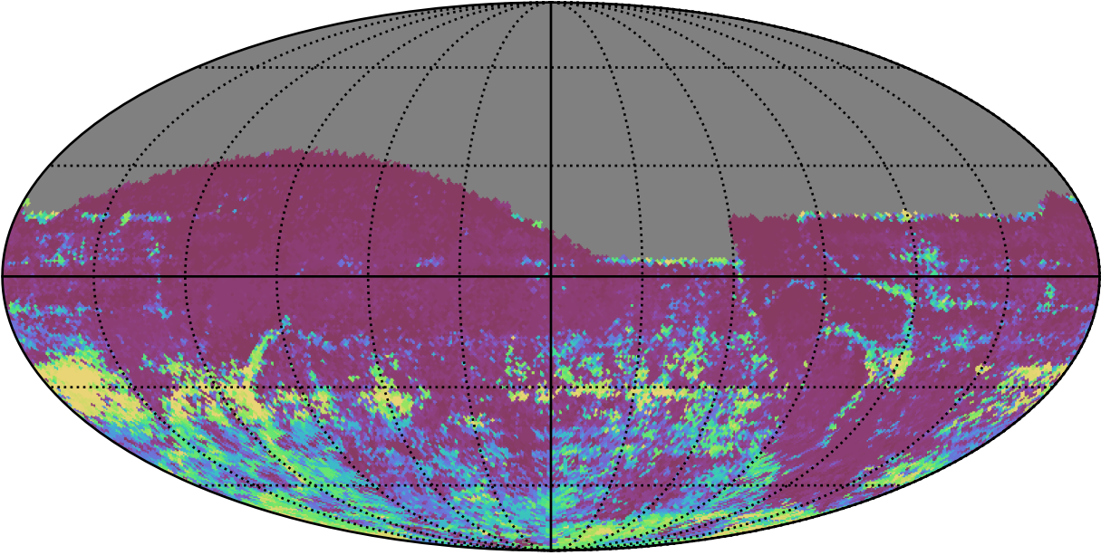
roll_uniform_eh_acc0.5_mjdp0_v3.4_10yrs All sky r band: 75th Percentile Intranight Timespan
