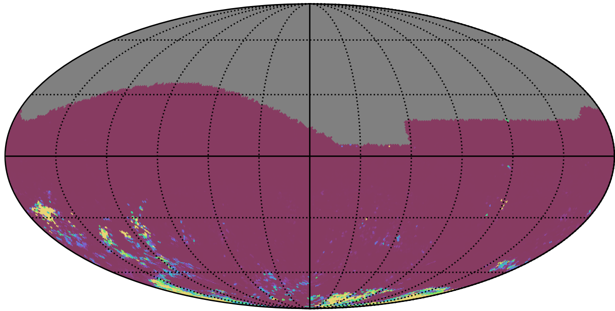
roll_uniform_eh_acc0.5_mjdp0_v3.4_10yrs All sky gr bands: 75th Percentile Intranight Timespan
