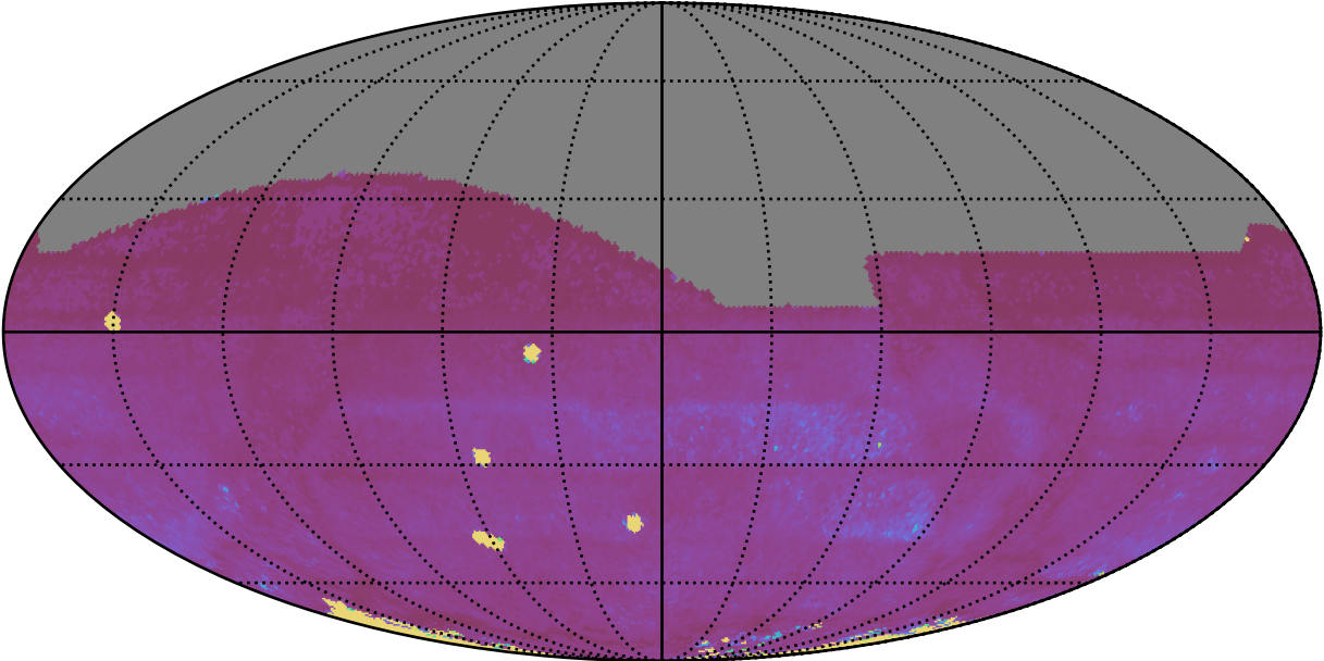
roll_uniform_eh_acc0.5_mjdp0_v3.4_10yrs All sky all bands: 75th Percentile Intranight Timespan
