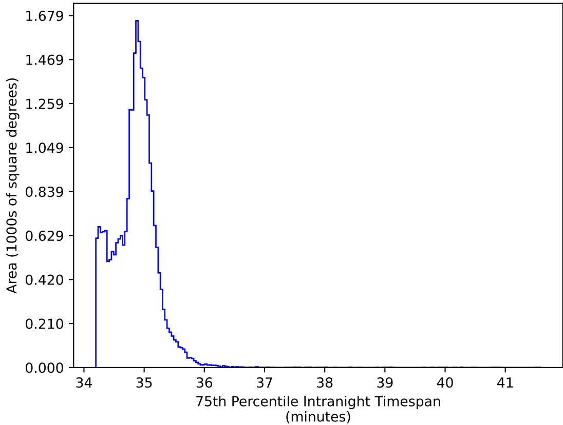
roll_uniform_eh_acc0.5_mjdp0_v3.4_10yrs All sky: 75th Percentile Intranight Timespan
