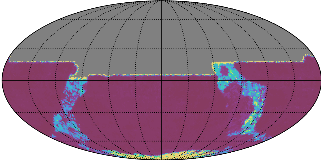
roll_uniform_eh_acc0.5_mjdp0_v3.4_10yrs All sky y band: 20thPercentile Inter-Night Gap
