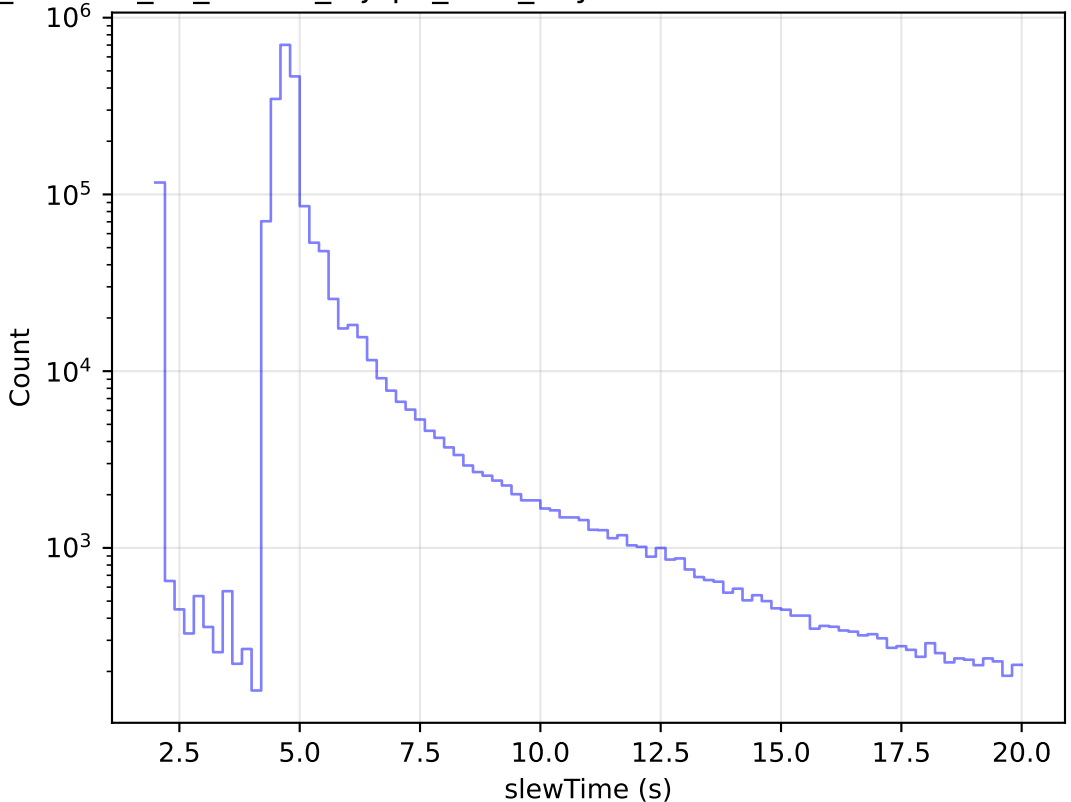
roll_uniform_eh_acc0.5_mjdp0_v3.4_10yrs All visits: Zoom Slew Time Histogram
