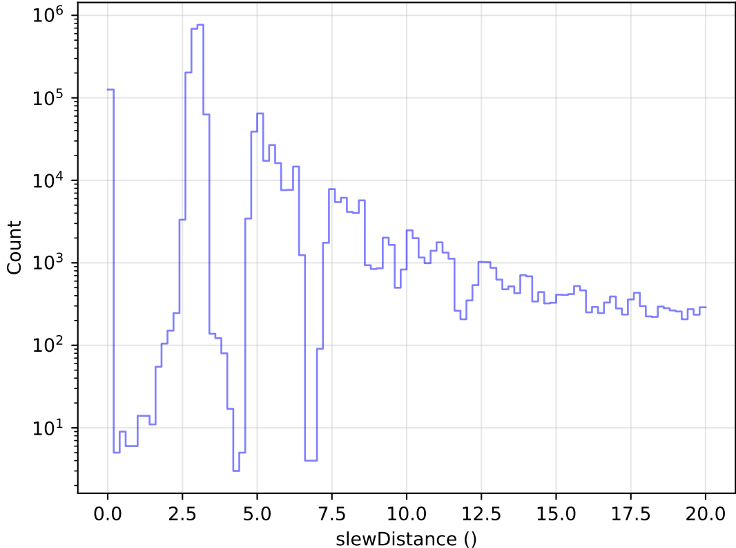
roll_uniform_eh_acc0.5_mjdp0_v3.4_10yrs All visits: Zoom Slew Distance Histogram
