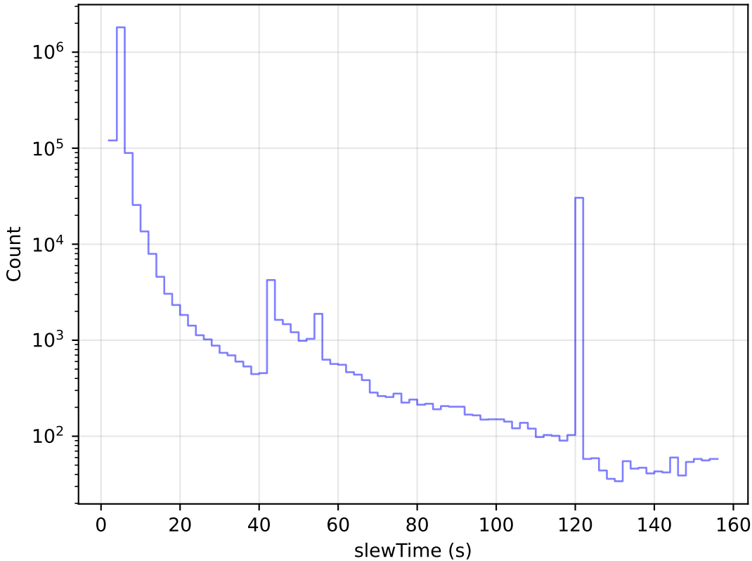
roll_uniform_eh_acc0.5_mjdp0_v3.4_10yrs All visits: Slew Time Histogram
