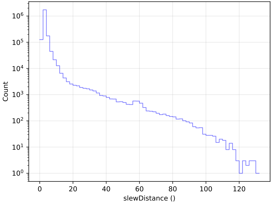
roll_uniform_eh_acc0.5_mjdp0_v3.4_10yrs All visits: Slew Distance Histogram
