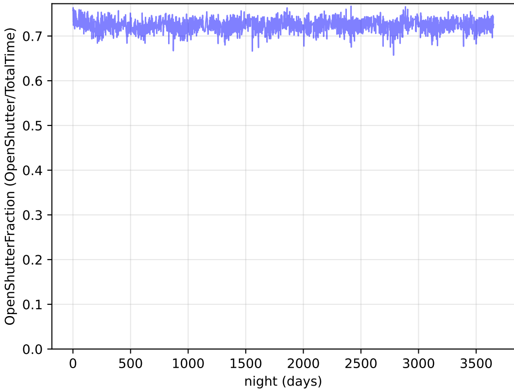
roll_uniform_eh_acc0.5_mjdp0_v3.4_10yrs : OpenShutterFraction
